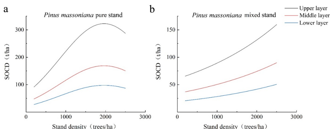
Figure 1. SOCD at different depths and stand densities. (a) SOCD at different depths and different stand densities in pure P. massoniana stands; (b) SOCD at different depths and different stand densities in mixed P. massoniana stand.
