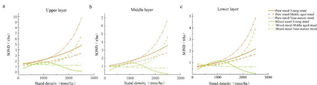
Figure 4. SOND with different stand densities and different age groups at different depths in pure and mixed P. massoniana stands. (a) SOND in the upper soil layer with different stand densities and different age groups in mixed and pure P. massoniana stands; (b) SOND in the middle soil layer with different stand densities and different age groups in mixed and pure P. massoniana stands; (c) SOND in the lower soil layer with different stand densities and different age groups in mixed and pure P. massoniana stands.
