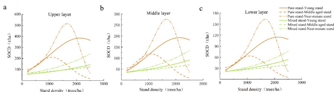
Figure 3. SOCD with different stand densities and different age groups at different depths in pure and mixed P. massoniana stands. (a) SOCD in the upper soil layer with different stand densities and different age groups in mixed and pure P. massoniana stands; (b) SOCD in the middle soil layer with different stand densities and different age groups in mixed and pure P. massoniana stands; (c) SOCD in the lower soil layer with different stand densities and different age groups in mixed and pure P. massoniana stands.
